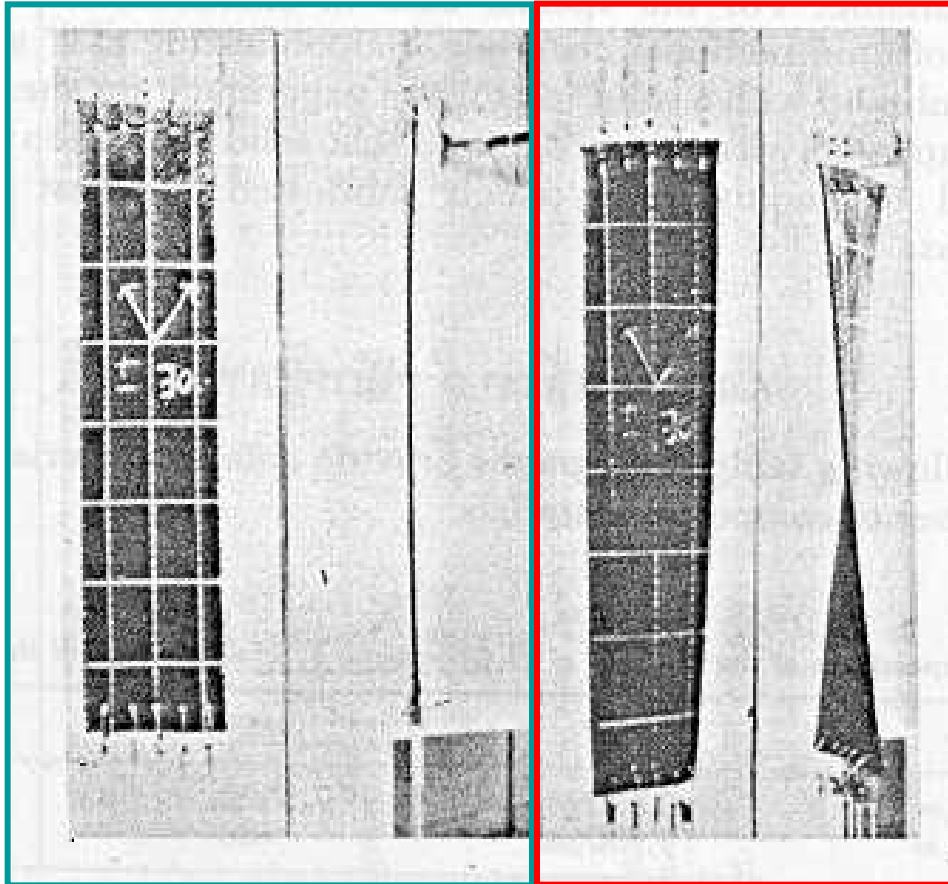
Un-deformed laminate
